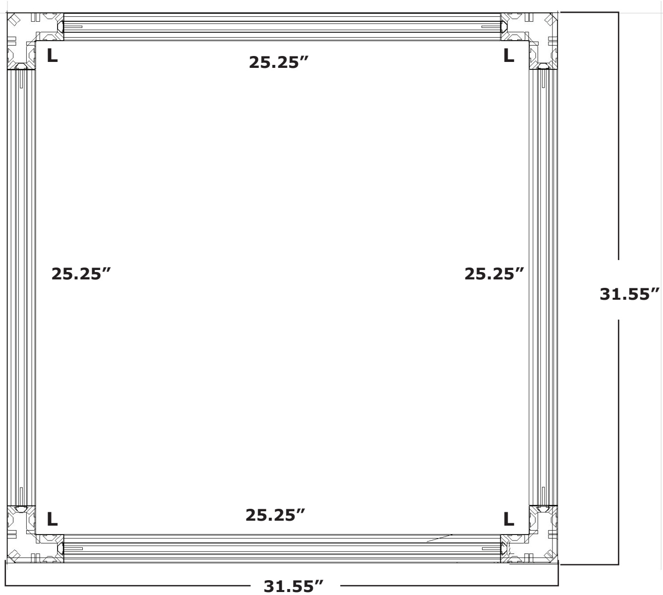
Vertical Extrusion = 94"
